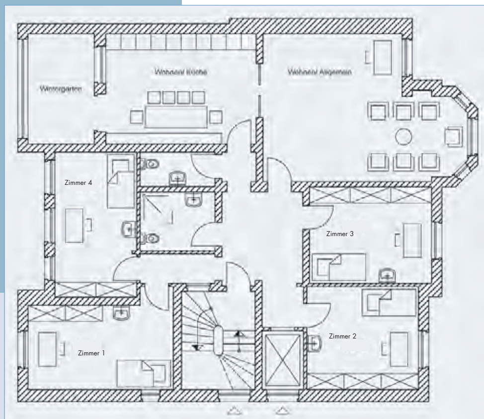
Grundriß Erdgeschoss.
